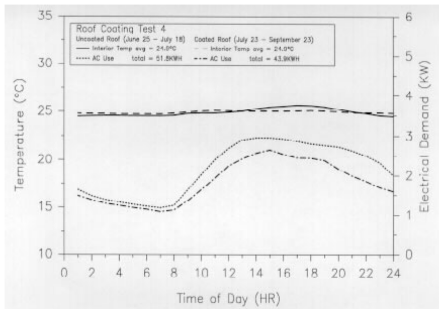
Figure 4a. Site 4 AC electricity use and interior air temperatures before and after coating.
