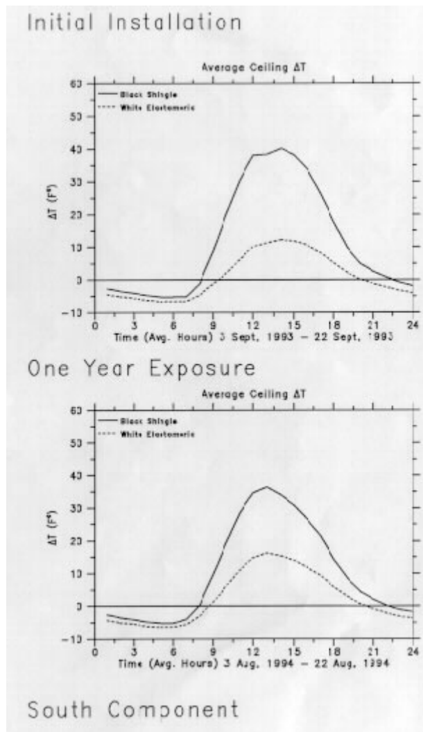
Figure 7. Measured change in ceiling heat flux from white vs. black shingle roof over a one-year period. (All four graphs).
