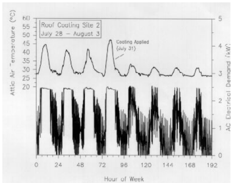
Figure 1b. Site 2 attic temperatures and AC load profiles during week of roof coating.
