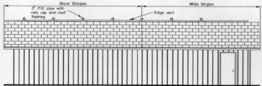
North Side Elevation
