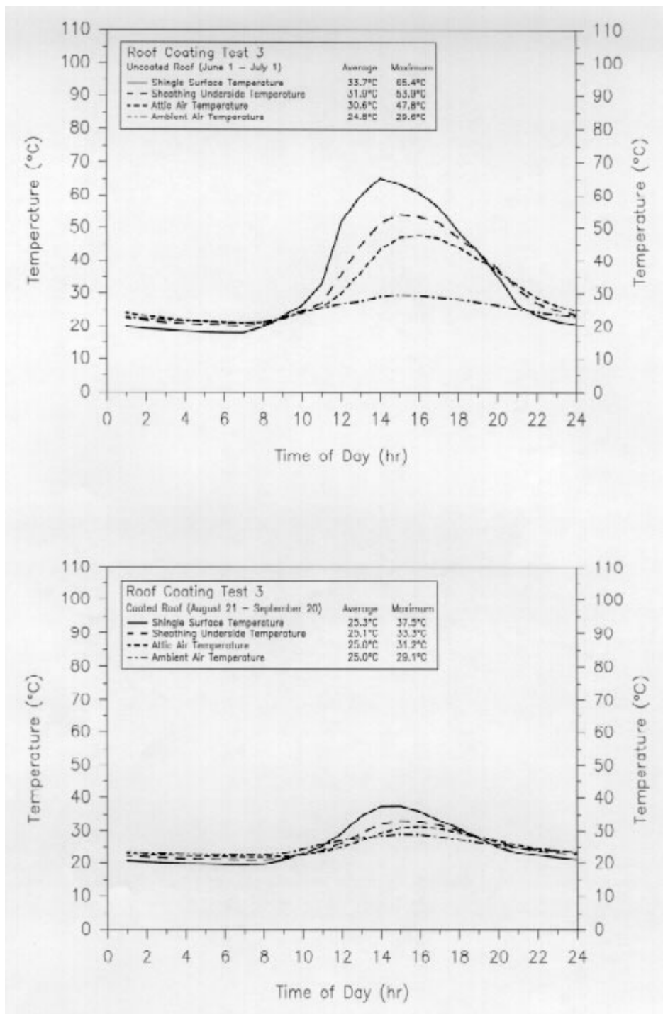
Figure 3b. Site 3 (asphalt single roof) hourly average temperatures a) uncoated, b) after coating.
